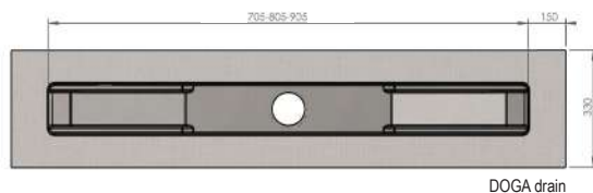
DOGA drain
